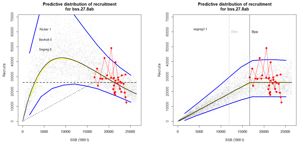
Figure 1. Sea bass in divisions 8.a–b; IBPBass 2018. Stock–recruitment relationship.
