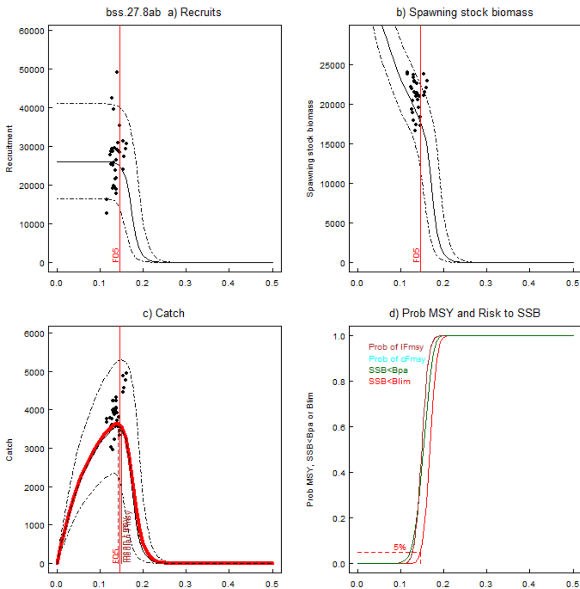
Figure 2. Sea bass in divisions 8.a-b; IBPBass 2018. Eqsim summary plot without B_{trigger} . Panels a to c: historic values (dots) median (solid black) and 90% intervals (dotted black) recruitment, SSB and landings for exploitation at fixed values of F . Panel c also shows mean landings (red solid line). Panel d shows the probability of SSB < B_{lim} (red), SSB < B_{pa} (green) and the cumulative distribution of F_{MSY} based on yield as landings (brown).
