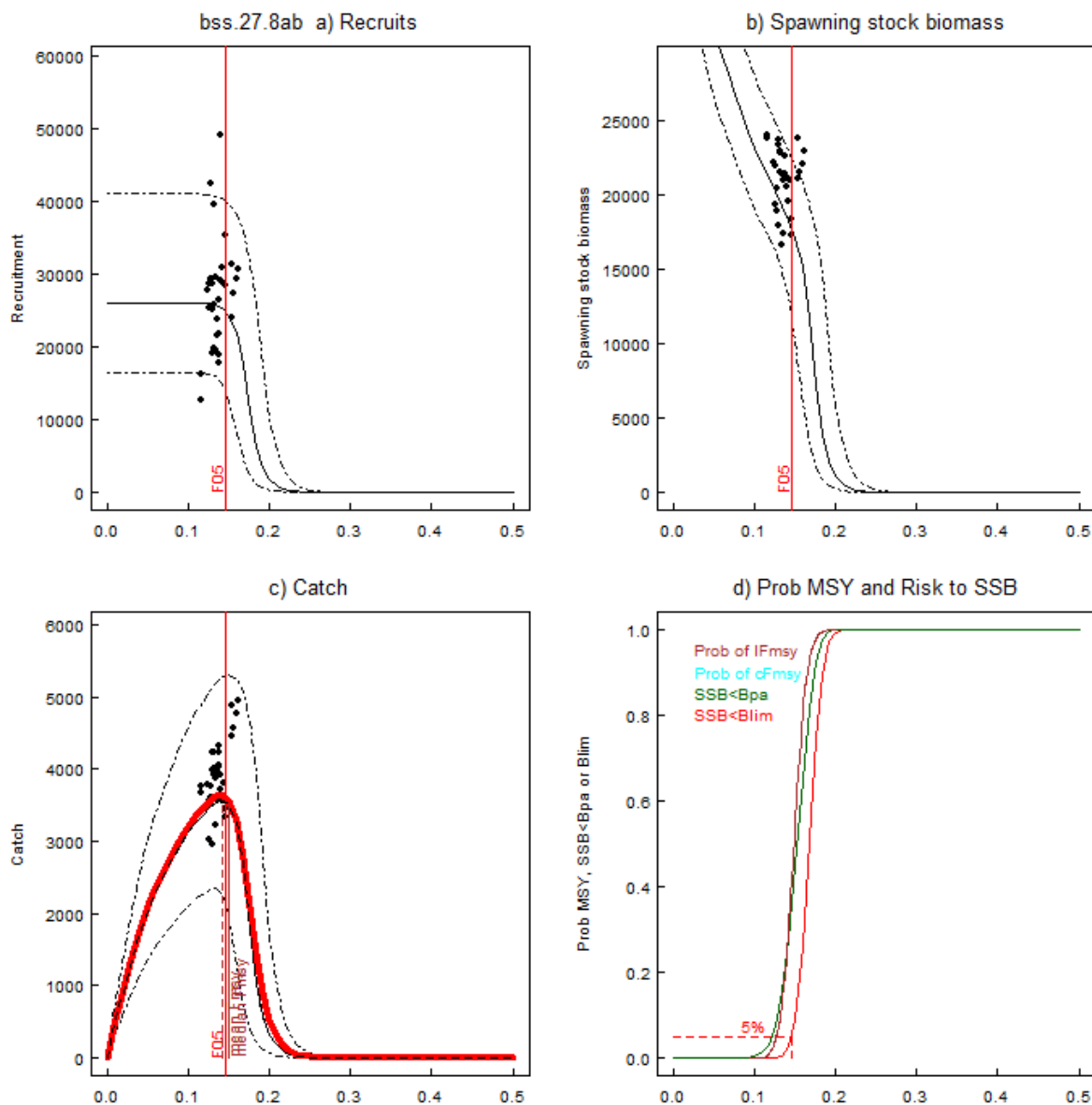
Figure 7. Eqsim summary plot without B_{trigger} . Panels a to c: historic values (dots) median (solid black) and 90% intervals (dotted black) recruitment, SSB and landings for exploitation at fixed values of F. Panel c also shows mean landings (red solid line). Panel d shows the probability of SSB < B_{lim} (red), SSB < B_{pa} (green) and the cumulative distribution of F_{MSY} based on yield as landings (brown).
