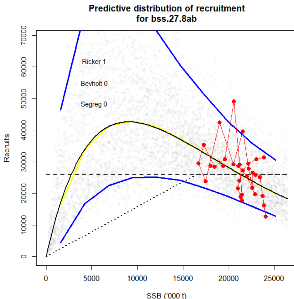
Figure 7. Sea bass in divisions 8.a–b; IBPBass 2018. Predictive distribution of recruitment.
