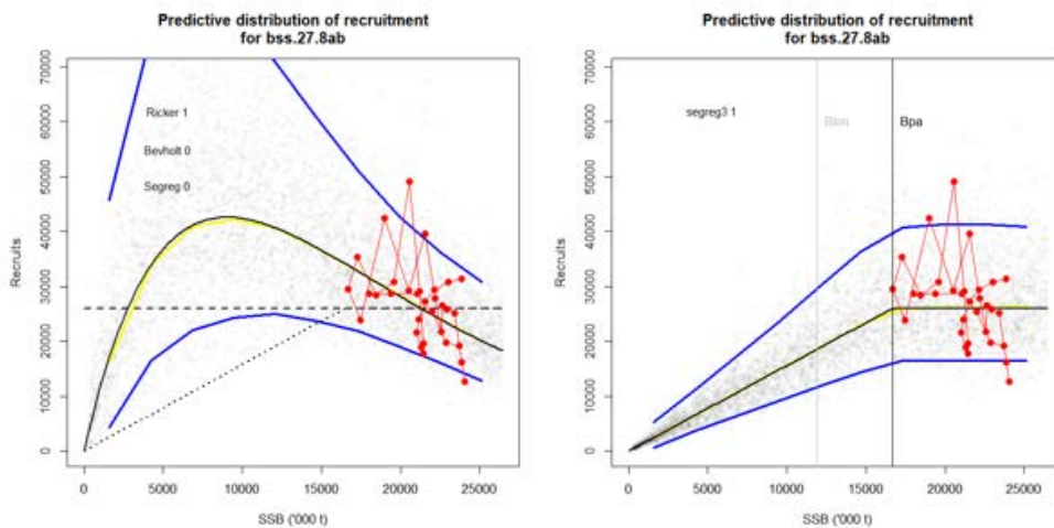
Figure 6. Stock–recruitment relationship for the seabass in divisions 8.ab.
