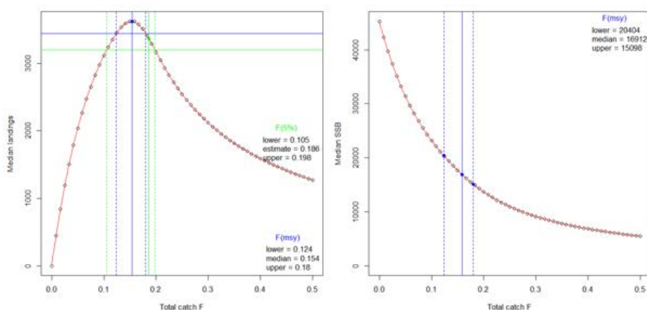
Figure 9. Eqsim median landings yield curve with estimated reference points with B_{trigger} . Blue lines: F_{MSY} estimate (solid) and range at 95% of maximum yield (dotted). Green lines: F(5\%) estimate (solid) and range at 95% of yield implied by F(5\%) (Dotted).
