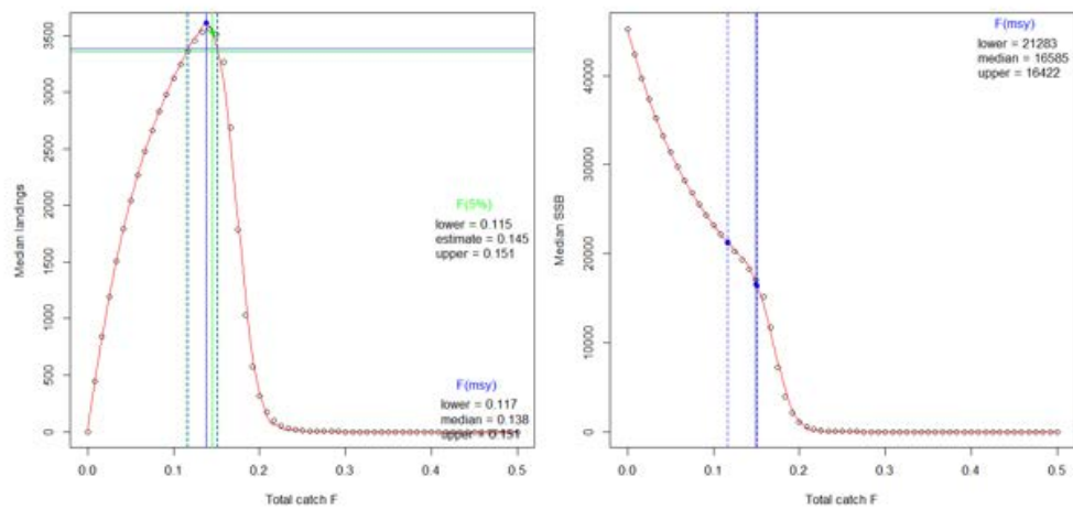
Figure 8. Left) Eqsim median landings yield curve with estimated reference points without B_{trigger} . Blue lines: F_{MSY} estimate (solid) and range at 95% of maximum yield (dotted). Green lines: F(5\%) estimate (solid) and range at 95% of yield implied by F(5\%) (Dotted). Right) Eqsim median SSB curve with estimated reference points without B_{trigger} . Blue dots: lower and upper SSB corresponding to lower and upper F_{MSY} .
