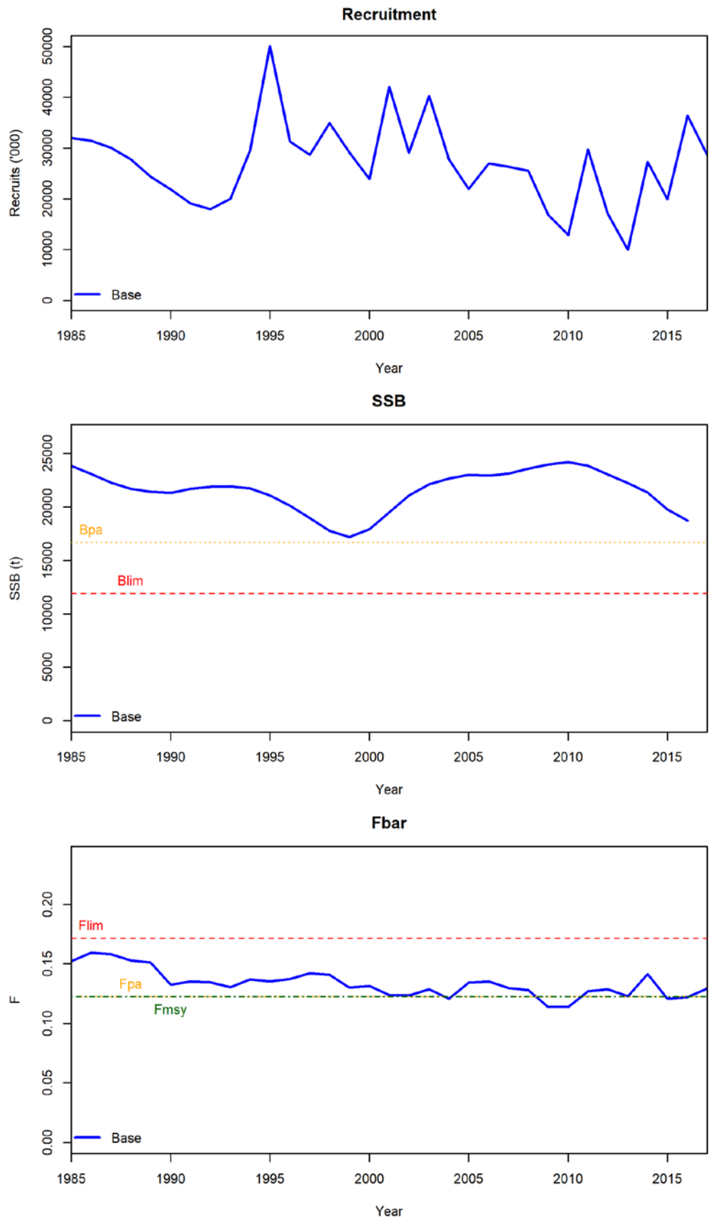
Figure 10. Recruitment, SSB and F_{bar} time-series with IBP2018 biological reference points.
