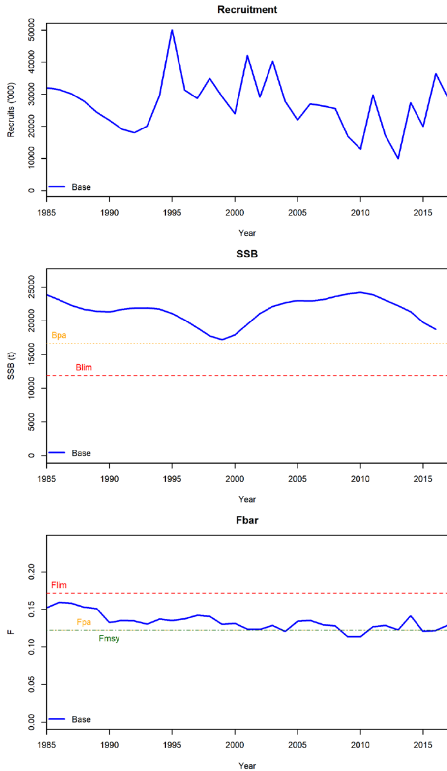
Figure 5. Sea bass in divisions 8.a-b; IBPBass 2018. Recruitment, SSB and F_{bar} time-series with IBPBass 2018 biological reference points.
