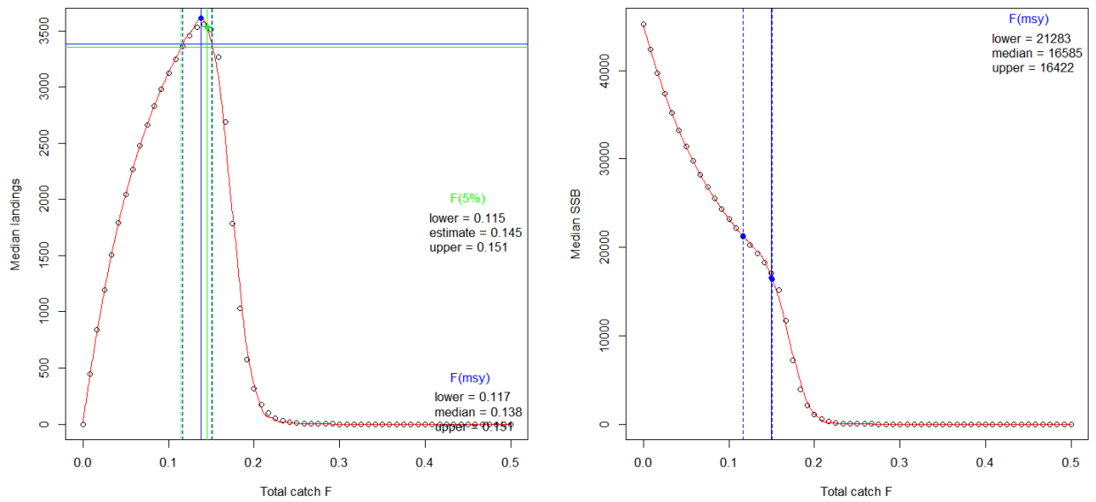
Figure 3. Sea bass in divisions 8.a–b; IBPBass 2018. Left plot is Eqsim median landings yield curve with estimated reference points without B_{trigger} . Blue lines: F_{MSY} estimate (solid) and range at 95% of maximum yield (dotted). Green lines: F(5\%) estimate (solid) and range at 95% of yield implied by F(5\%) (Dotted). Right plot is Eqsim median SSB curve with estimated reference points without B_{trigger} . Blue dots: lower and upper SSB corresponding to lower and upper F_{MSY} .
