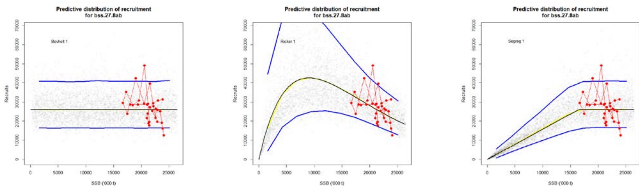
Figure 6. Sea bass in divisions 8.a-b; IBPBass 2018. Fits.
