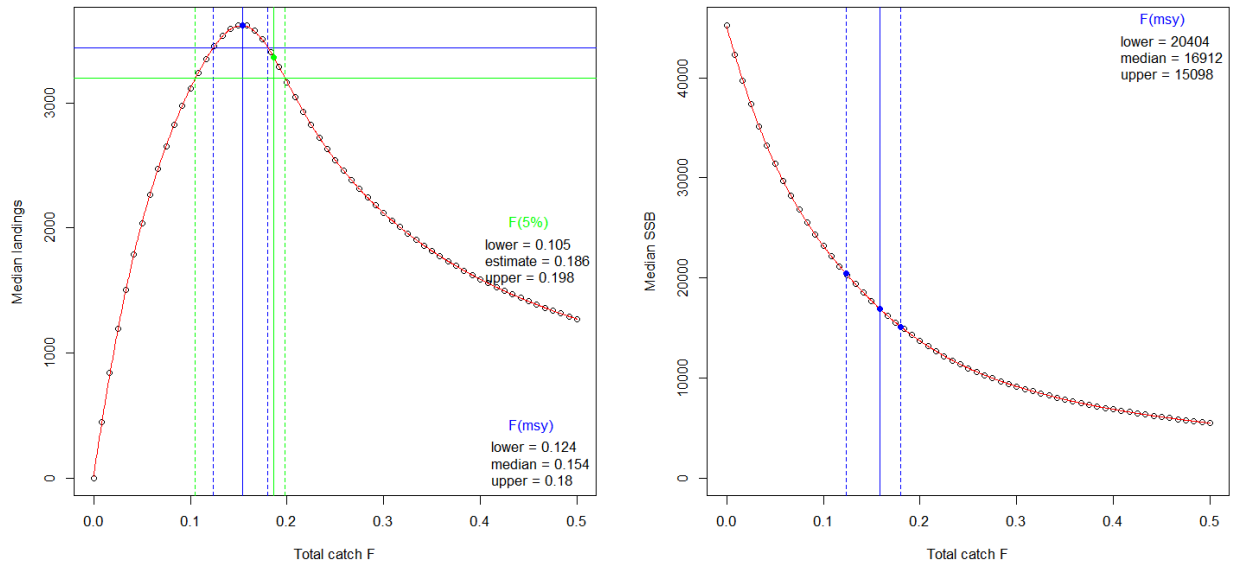
Figure 4. Sea bass in divisions 8.a–b; IBPBass 2018. Eqsim median landings yield curve with estimated reference points with B_{trigger} . Blue lines: F_{MSY} estimate (solid) and range at 95% of maximum yield (dotted). Green lines: F (5%) estimate (solid) and range at 95% of yield implied by F (5%) (Dotted).
