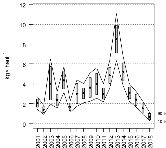
Figure 3 Ling in subareas 6–9, 12, and 14, and in divisions 3.a and 4.a. Estimated biomass index based on the Spanish Porcupine Bank survey (divisions 7.c and 7.k) for the years 2001–2018. Boxes mark the parametric based standard error of the stratified index. Lines mark bootstrap confidence intervals ( \alpha = 0.80 , bootstrap iterations = 1000).
