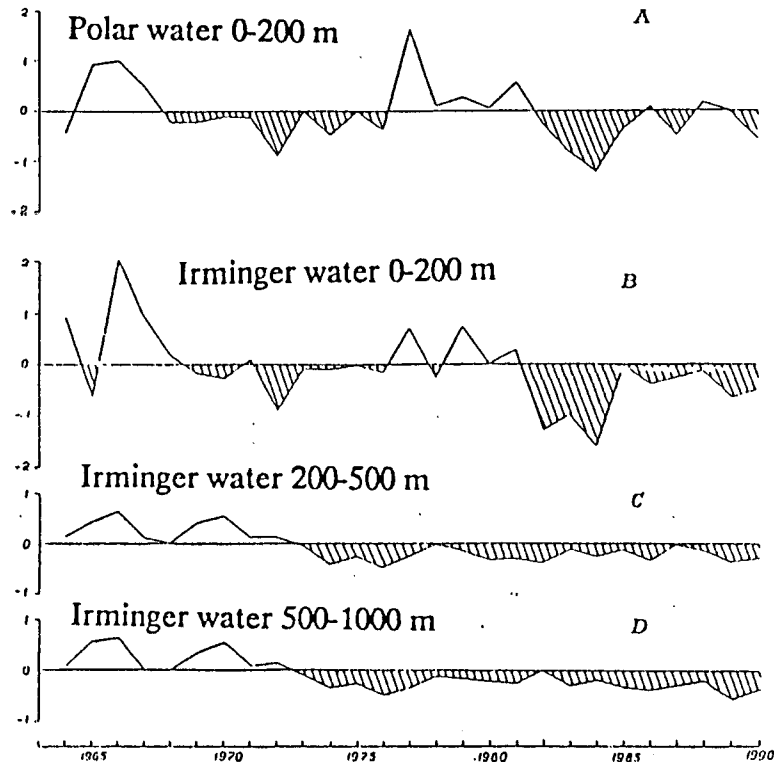
Fig. 13. Sea temperature off Newfoundland 1964-1990 (Borokov and Tevs 1991).
