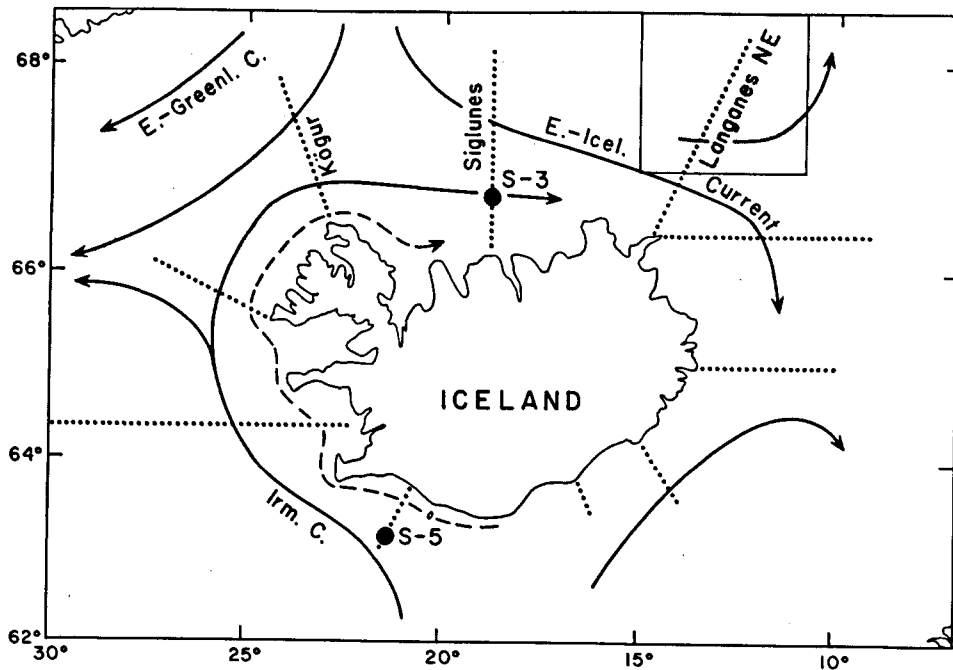
Fig. 2. Main ocean currents and location of standard hydrobiological sections in Icelandic waters. Selected areas and stations dealt with in the paper are indicated. (Malmberg and Kristmannsson 1992).
