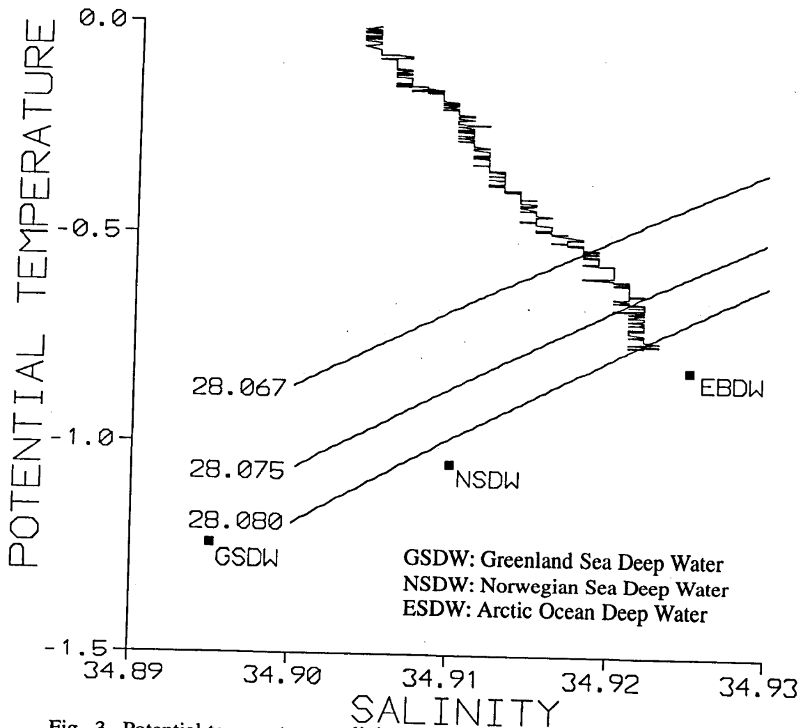
Fig. 3. Potential temperature - salinity diagram from a station of the southernmost section shown in Fig. 1. (Buch et al. 1992).
